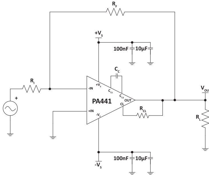
Figure 1: Typical Connection
