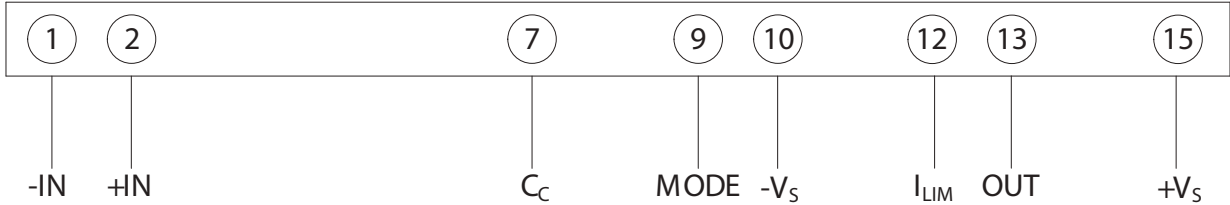
Figure 3: External Connections
