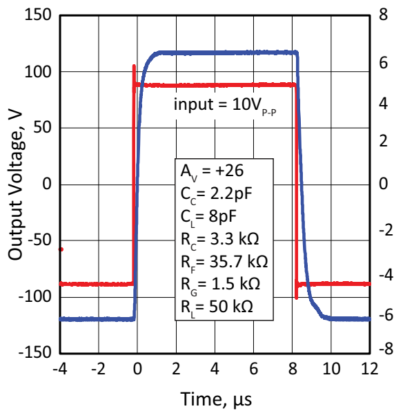
Figure 30: Transient Response
