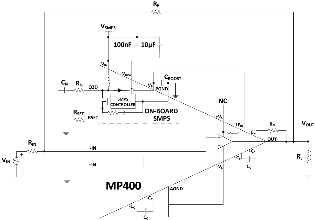
Figure 2: Typical Connection
